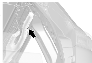
Curtain air bag module (LH and RH)
